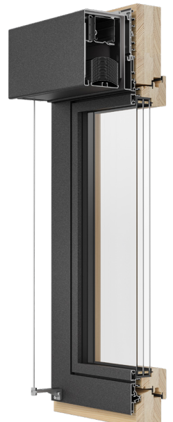
SYSTEM RAFA C-slat Rope guide
