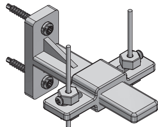
Bracing angle Combination
