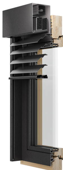
SYSTEM RAFE Z slat
