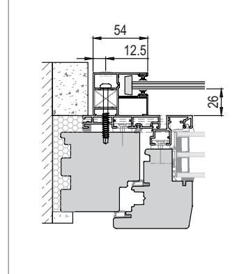
FS energy saving DT view
