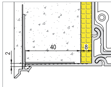
Detail plaster rail Plaster rail 40 mm
