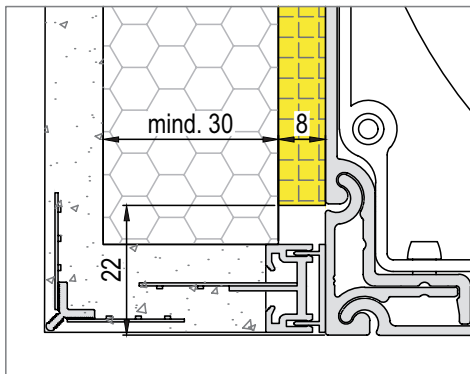
Detail of WDV connection Plaster rail 0 mm
