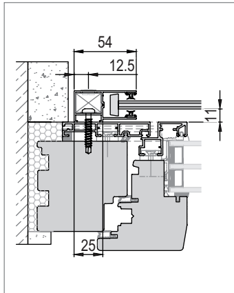
FS standard view
