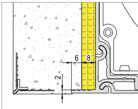
Detail plaster rail Plaster rail 6 mm
