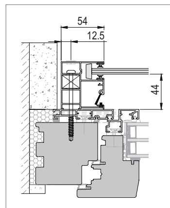
FS energy saving RO sight
