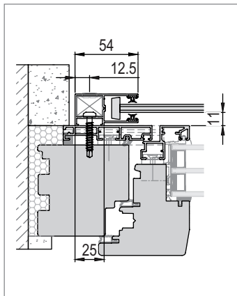
FS insect screen sight
