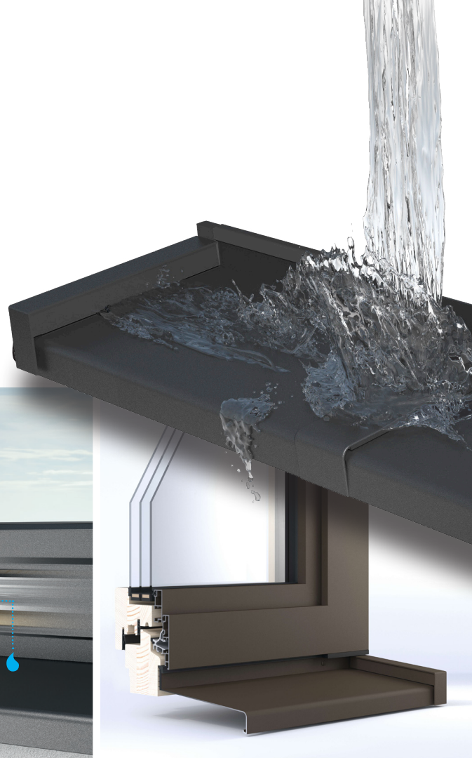
A Sealed sliding rib
