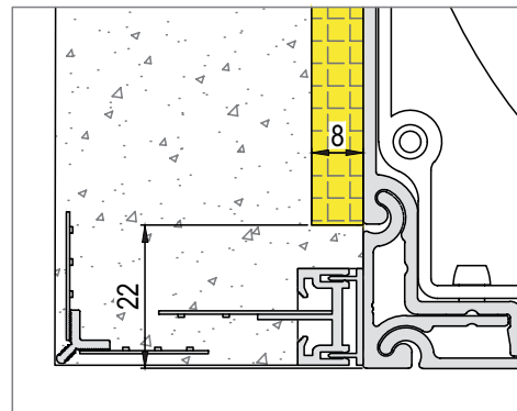
Detail plaster strip Plaster rail 0 mm
